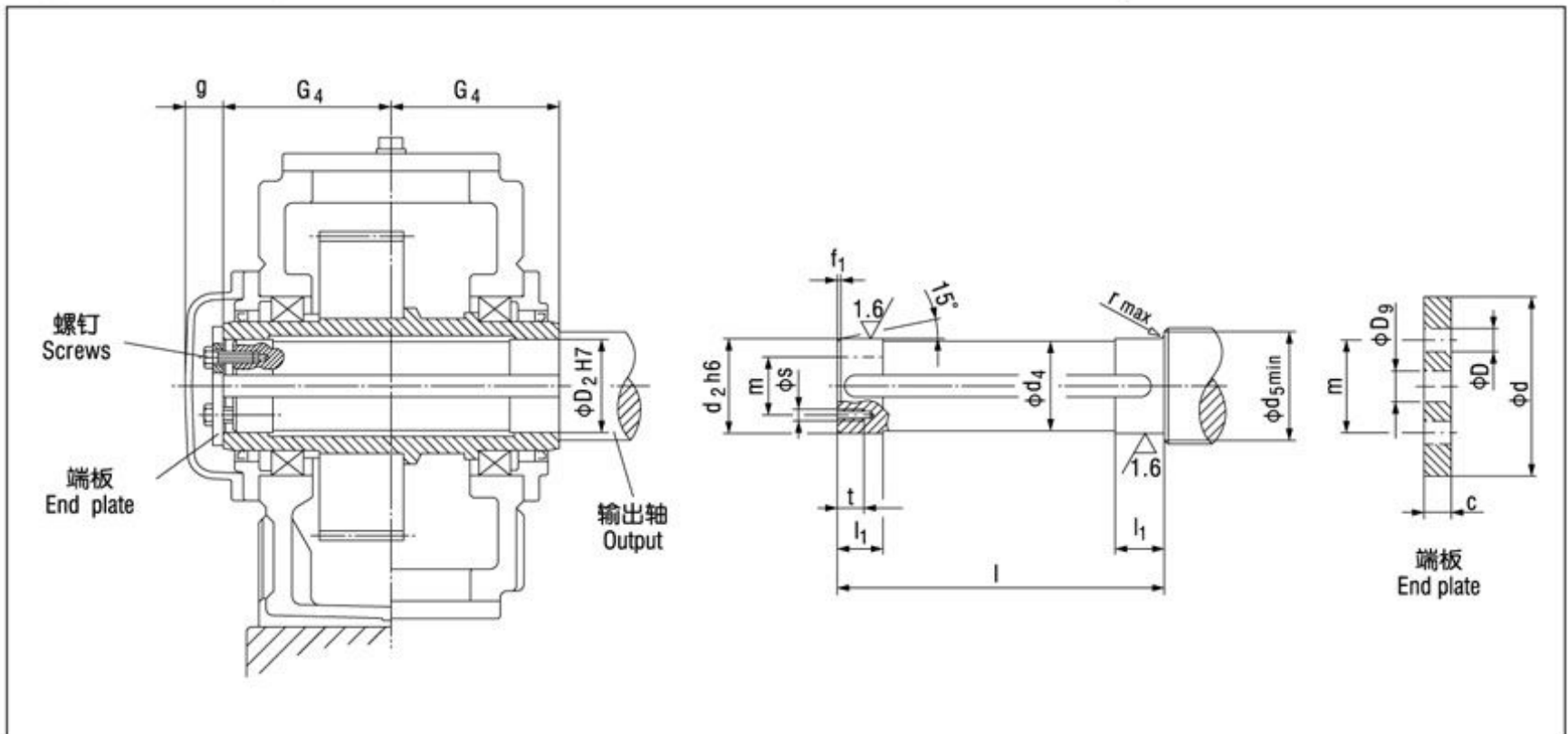
Hollow Shafts for flat key:
